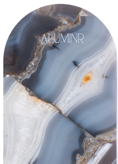
Grey Agate
