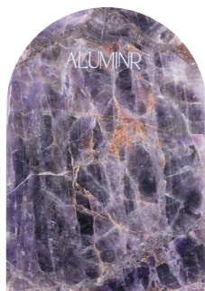
Amethyst
